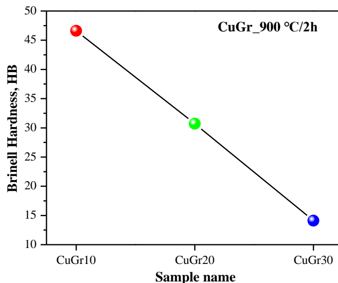
Figure 6. Graphite weight change of copper-graphite composite samples versus Brinell hardness.
